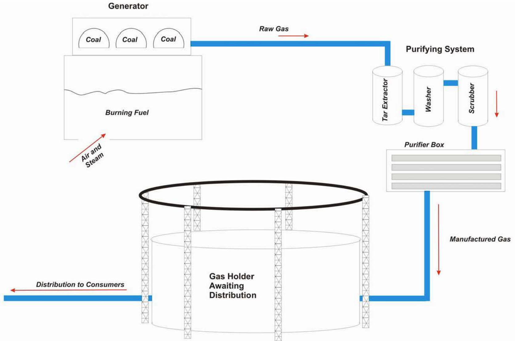
The Gas Manufacturing Process: Overview
