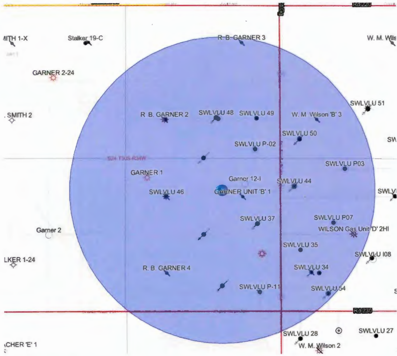
SWLVLU 45 AOR MAP
