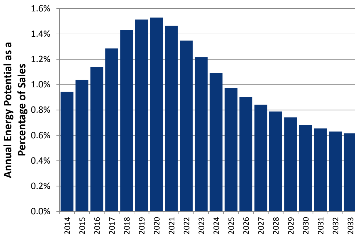
Figure 3-4. Incremental RAP as a % of Baseline Forecast Energy Sales – KCP&L MO
